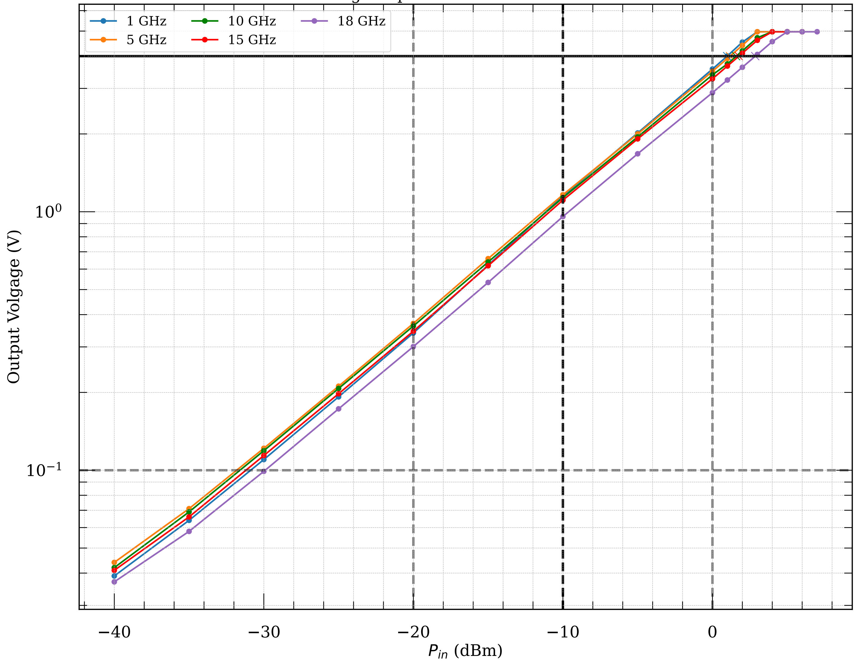
Measured voltage-to-power curve of detector module034v2
